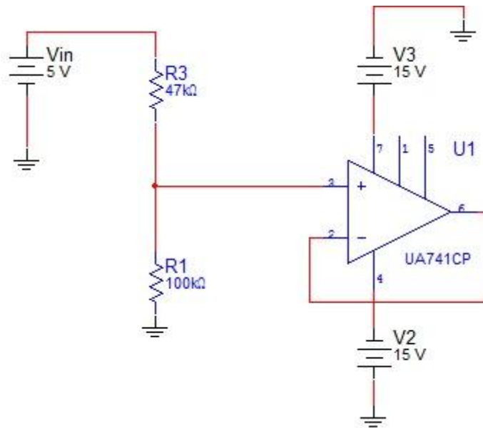
Figure 18: Voltage Divider Circuit for Force Sensing
