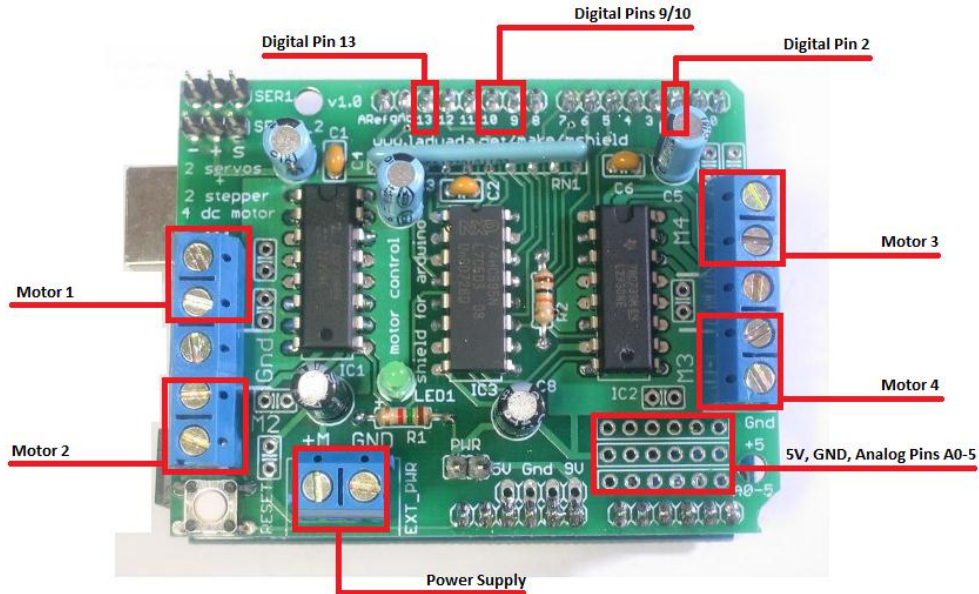
Figure 10. Adafuit Motor Shield Layout
