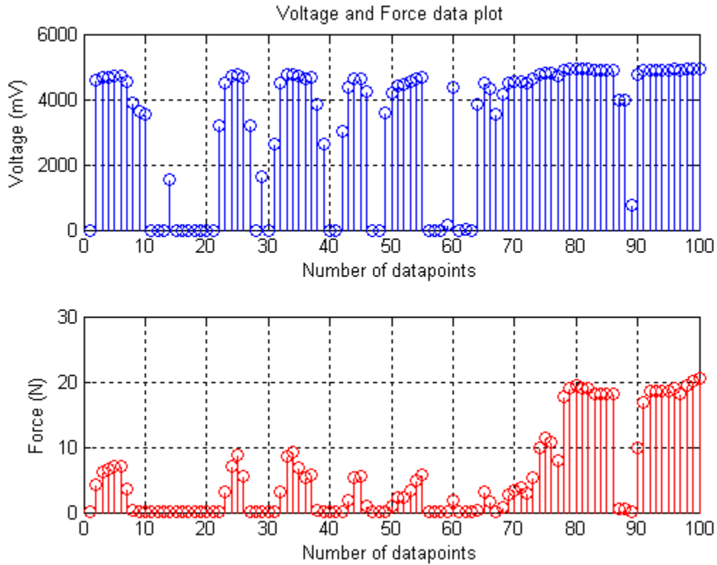
Figure 20: ball experiment sensor data
