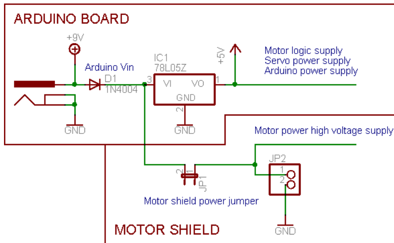
Figure 11. Adafuit Motor Shield Power Supply Wire Diagram
